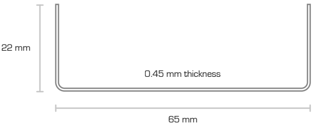
Track 65x22x0.45
