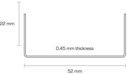
Track 52x22x0.45
