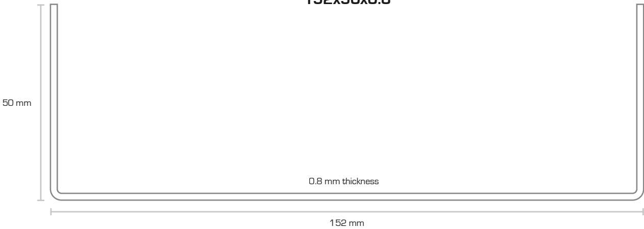
Track 152x50x0.8
