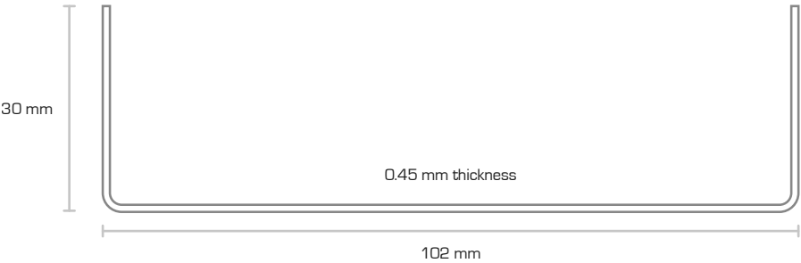
Track 102x30x0.45
